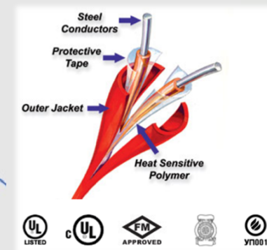
BlazeWire Detection (180°C)
