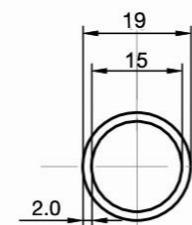
Heat sensitive tube (cross section)
