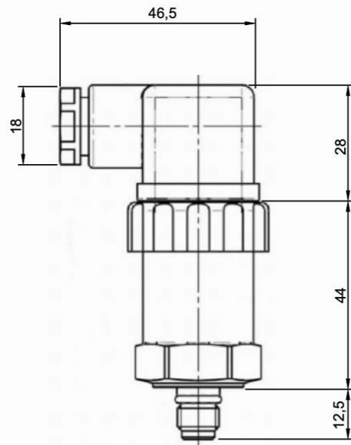
Pressure Switch APS001 (side view)
